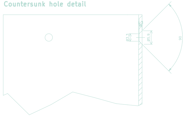
Countersunk hole detail
